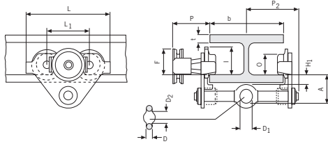
HTP/G, 500 - 5000 kg
